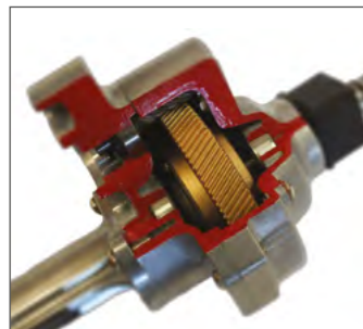
Limited Slip Differential Gearbox
